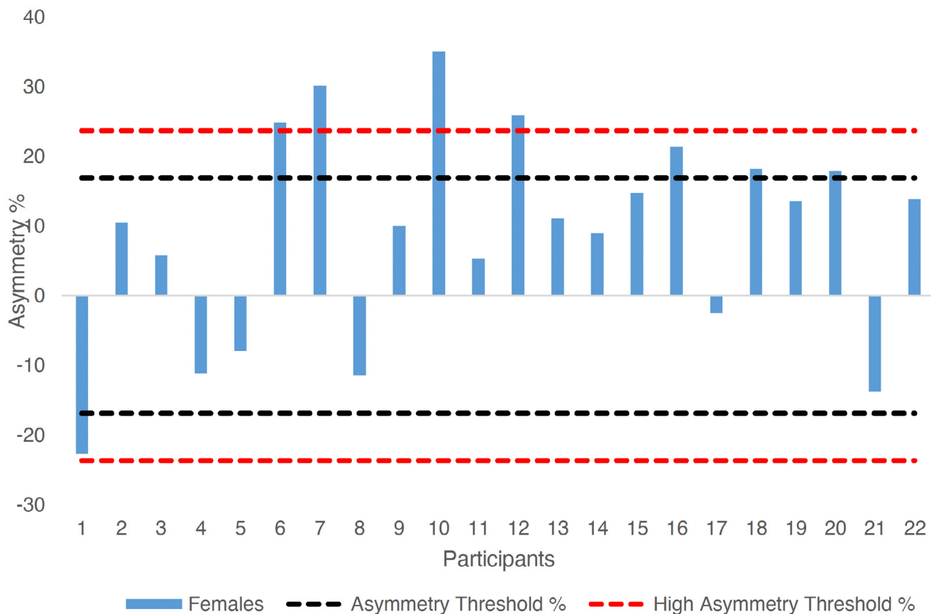
Figure 3. Individual inter-limb magnitude with direction asymmetry data for females for absolute eccentric HABd. Note: Above 0 asymmetry favours the dominant limb and below 0 indicates asymmetry favours the non-dominant limb.
